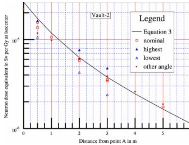
FIG. 4. (Color) Neutron dose equivalent along the maze of Vault-2. Data obtained with the meter orientation the same as at calibration are denoted nominal. The highest readings are usually at 45° clockwise from nominal as observed from above (closed triangle). The lowest readings are usually at 225° clockwise from nominal (open triangle). The other angle refers to the readings with the meter rotated 180° from nominal (diamonds).
